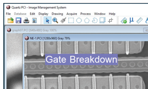
IMAGE ANNOTATION
